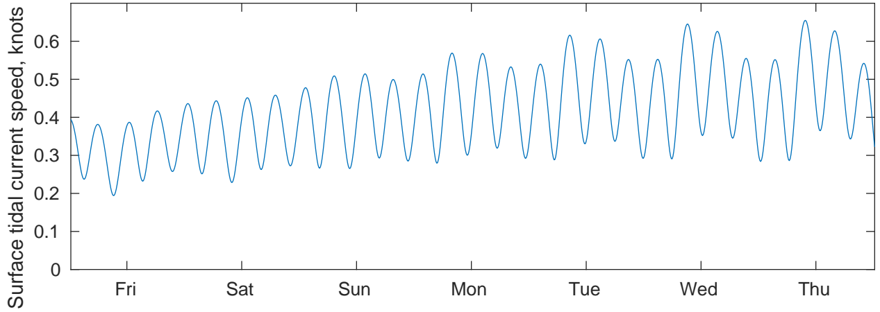
Tidal Currents and Heights for OCS-A 0538 at 20240418
